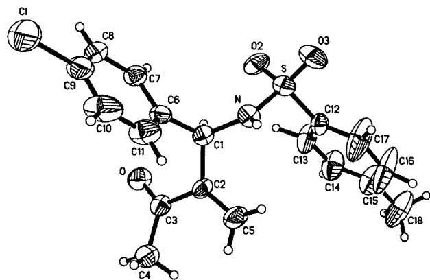
Figure 1. Crystal structure of 1e .
